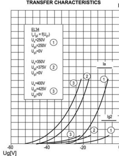
TRANSFER CHARACTERISTICS
